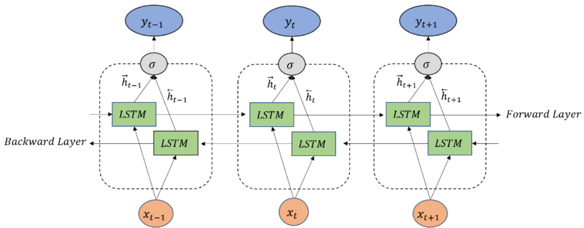
Gambar 3 Arsitektur Bi-LSTM [34]
